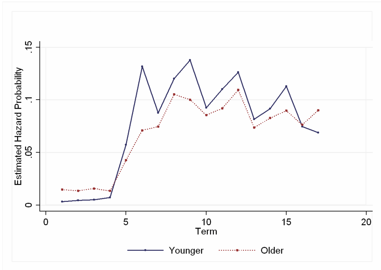
Figure 1: Sample Hazard of Completion by Age
